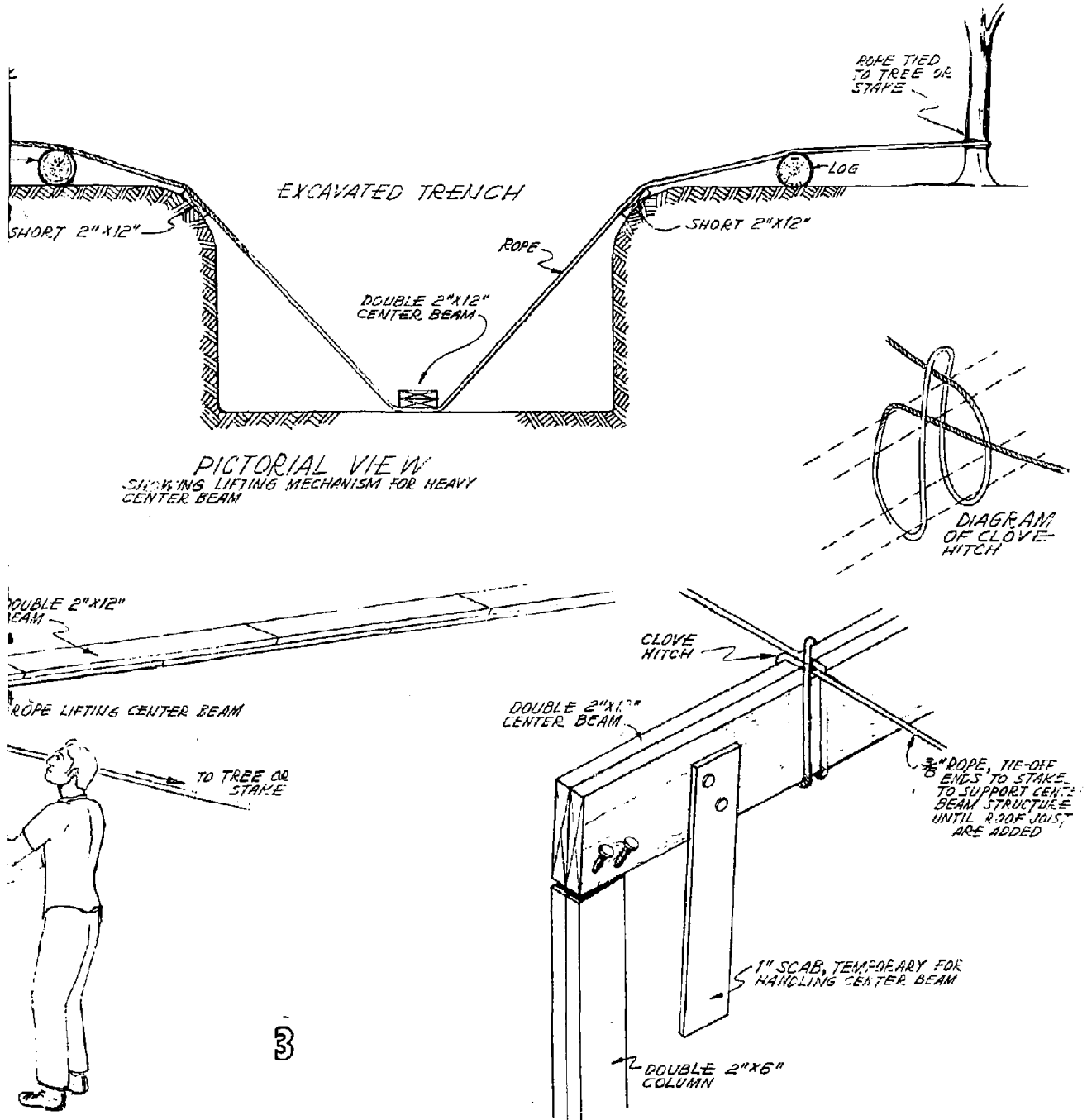
3.2. Trench Walls Underground Shelter, Construction Methods.
